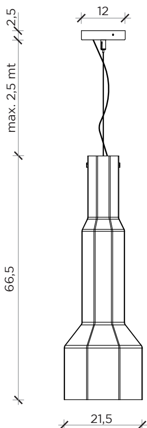
FRONTE | FRONT
