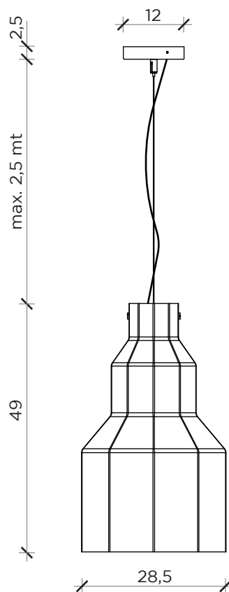
FRONTE | FRONT
