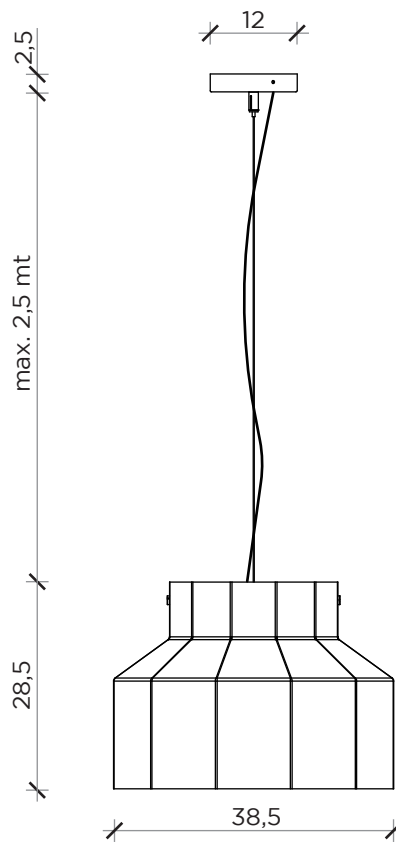
FRONTE | FRONT
